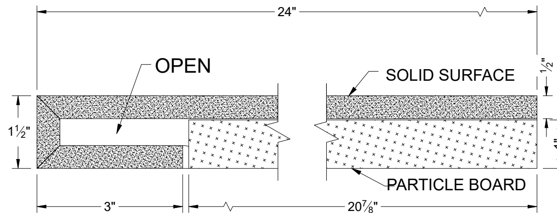
A 31 SECTION
