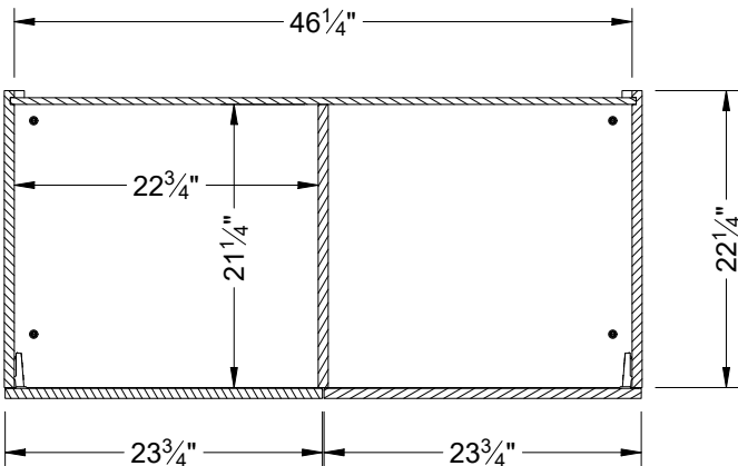
SECTION VIEW
