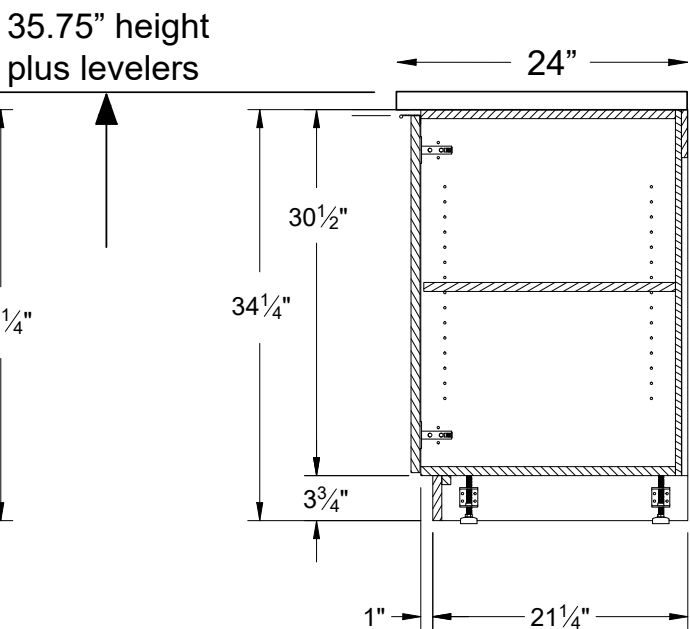
SECTION VIEW
