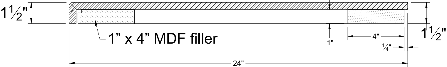
A 4 SECTION W/ BACKSPLASH 3" = 1' COUNTERTOP OPTIONS
